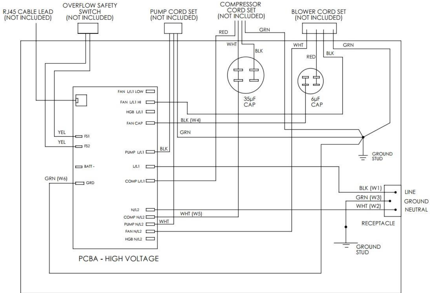
WIRING SCHEMATIC - PHD 200
